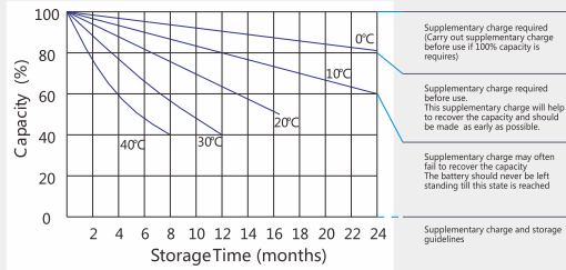
Storage characteristic
